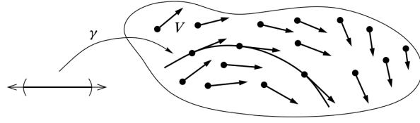
Figure 1: An integral curve of a vector field.
